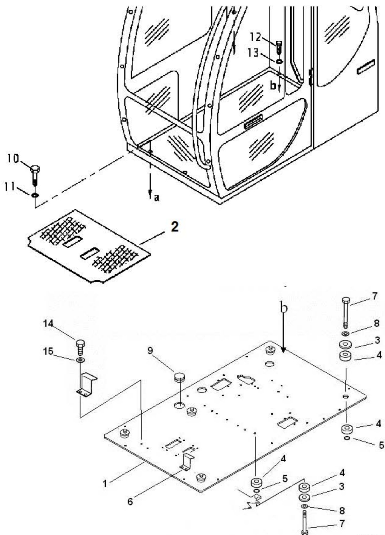
FIG: 5140 OPERATOR'S CAB, FLOOR FRAME
