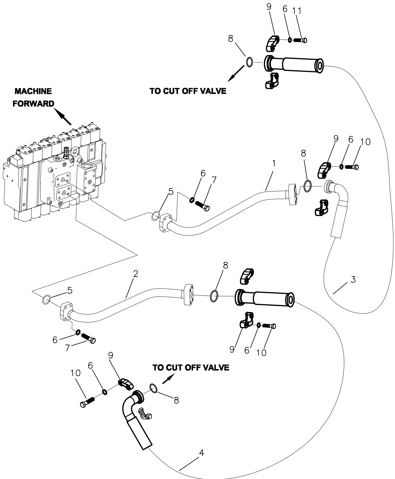
FIG. 6170 HYDRAULIC PIPING (CONTROL VALVE TO PUMP)
