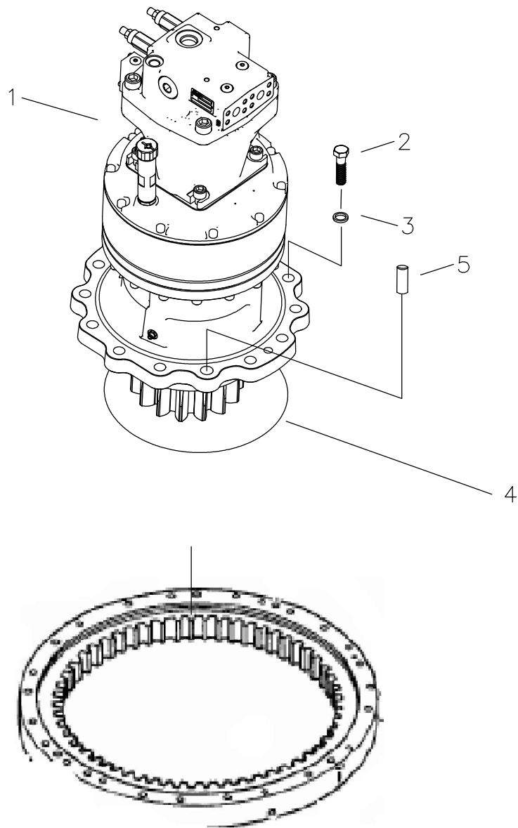
SWING CIRCLE
