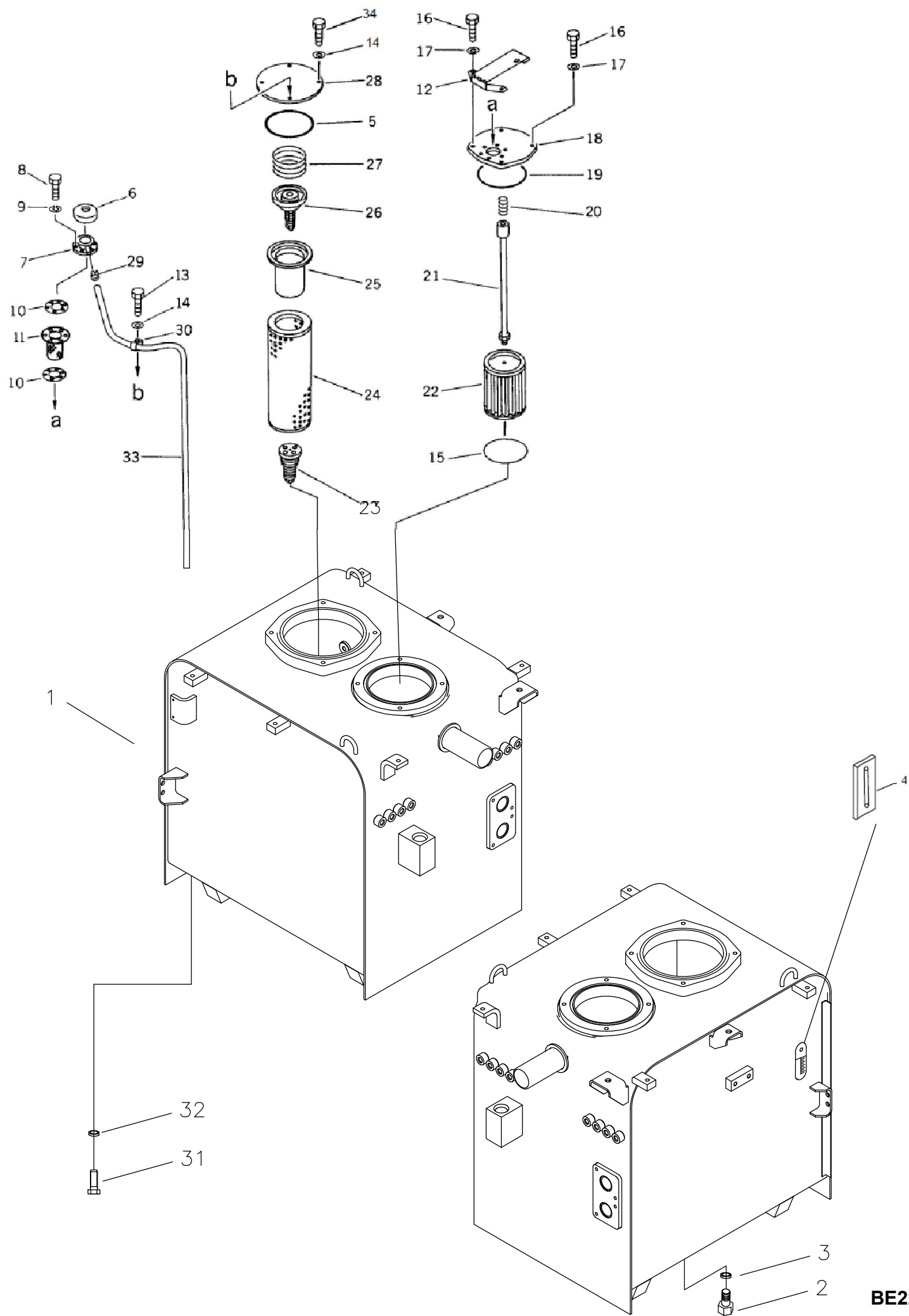
FIG. 6080 HYDRAULIC TANK
