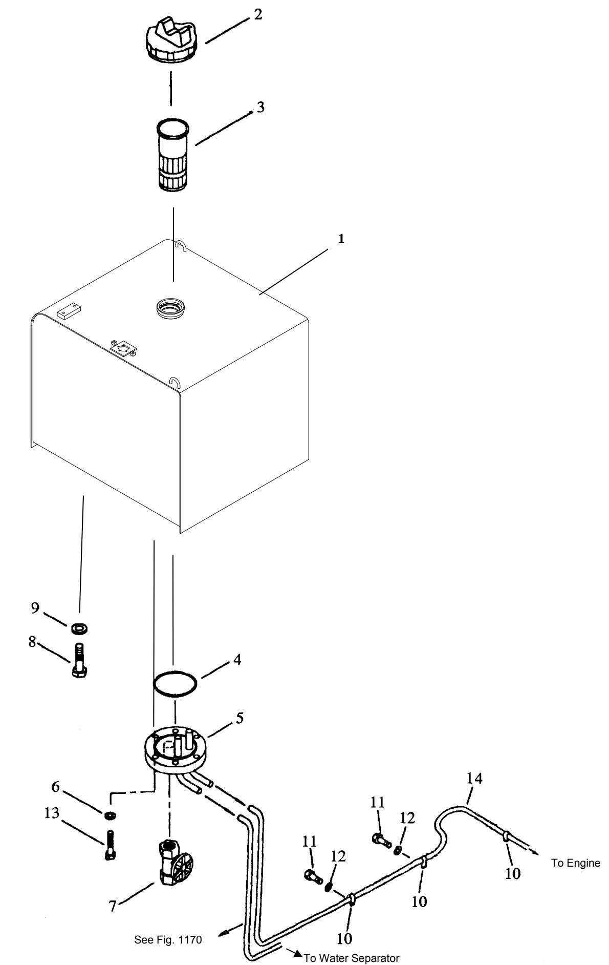
FIG. 1080 FUEL TANK
