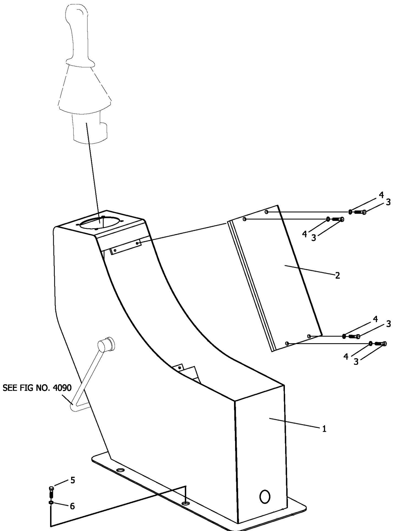
FIG. 4080 CONTROL STAND LH
