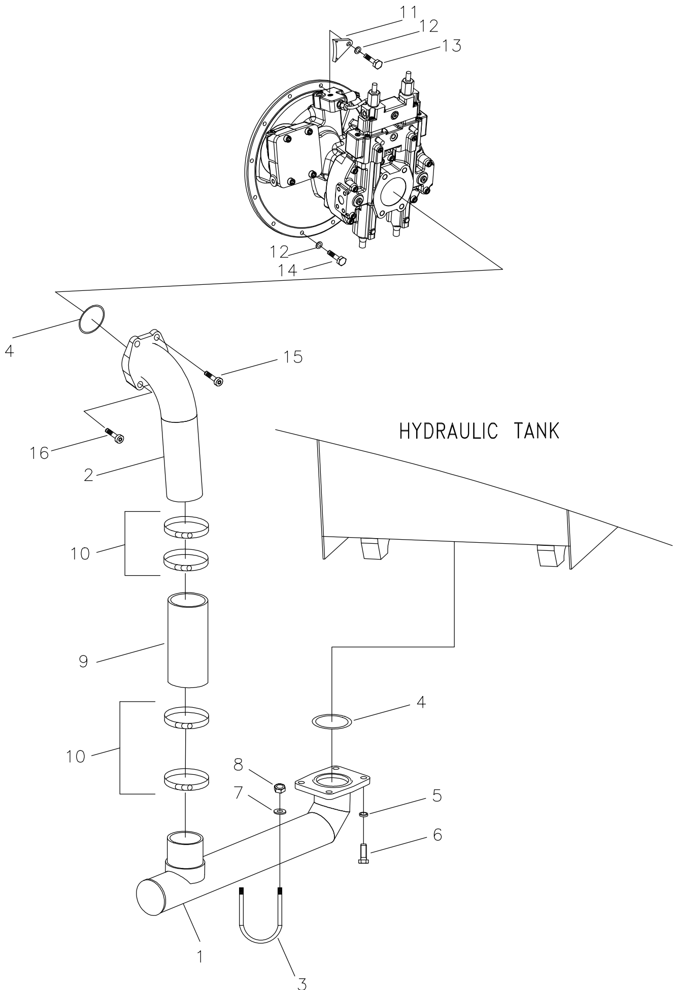
FIG. 6160 HYDRAULIC PIPING (TANK TO PUMP)
