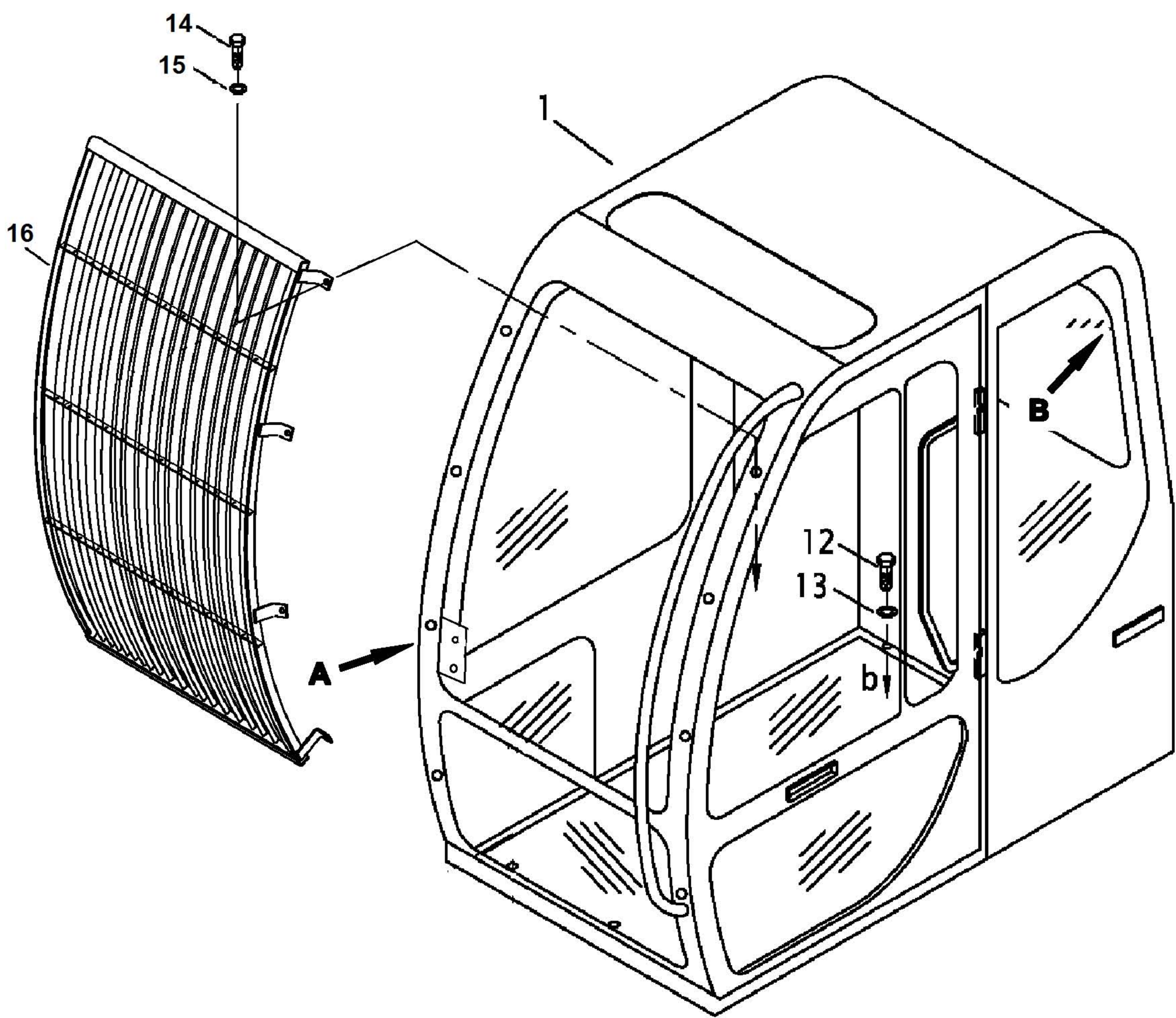
FIG 5071 OPERATOR'S CAB (1/2)
