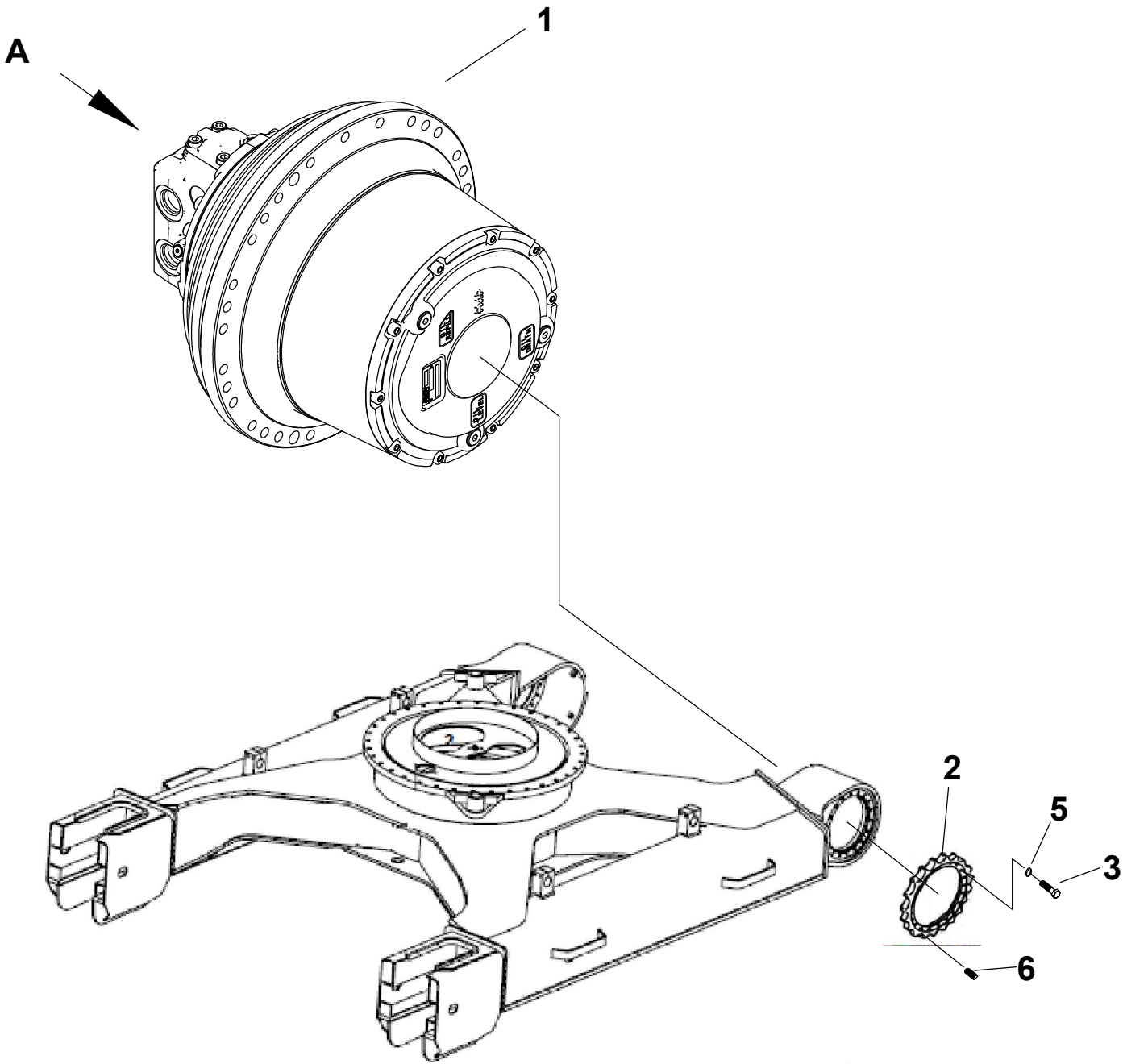
FIG. 2120 FINAL DRIVE WITH TRAVEL MOTOR
